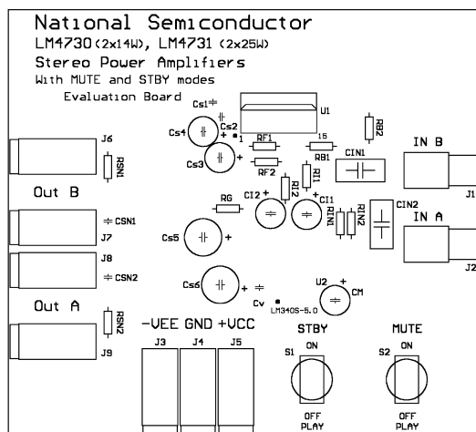
Figure 10. Silk Screen
