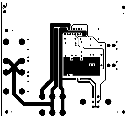
Figure 11. Top Layer
