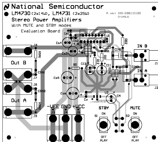
Figure 10. Silk Screen
